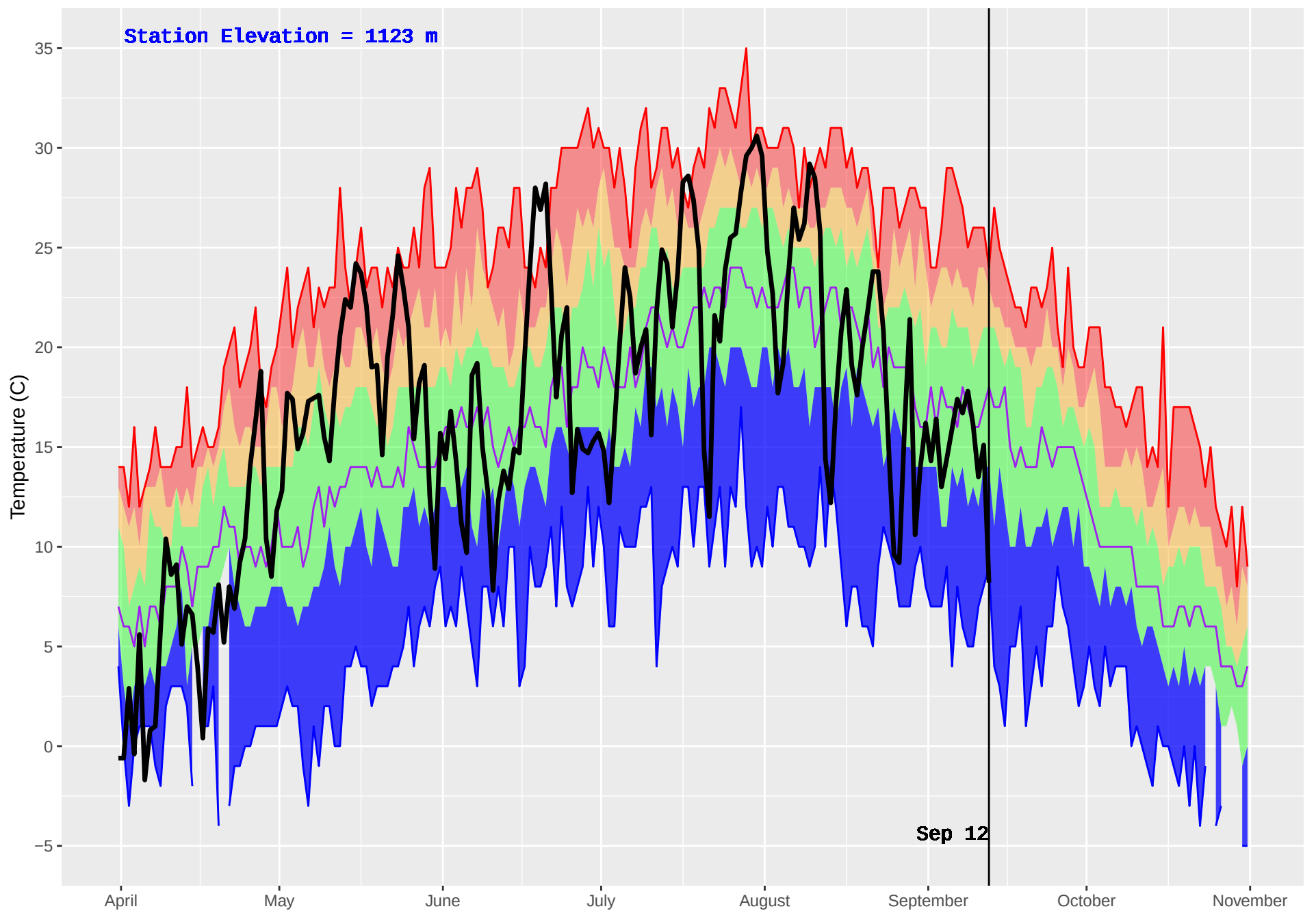
MCLEAN LAKE (311) : Historical (1987–2016) and Current (2018) Daily Temperature
