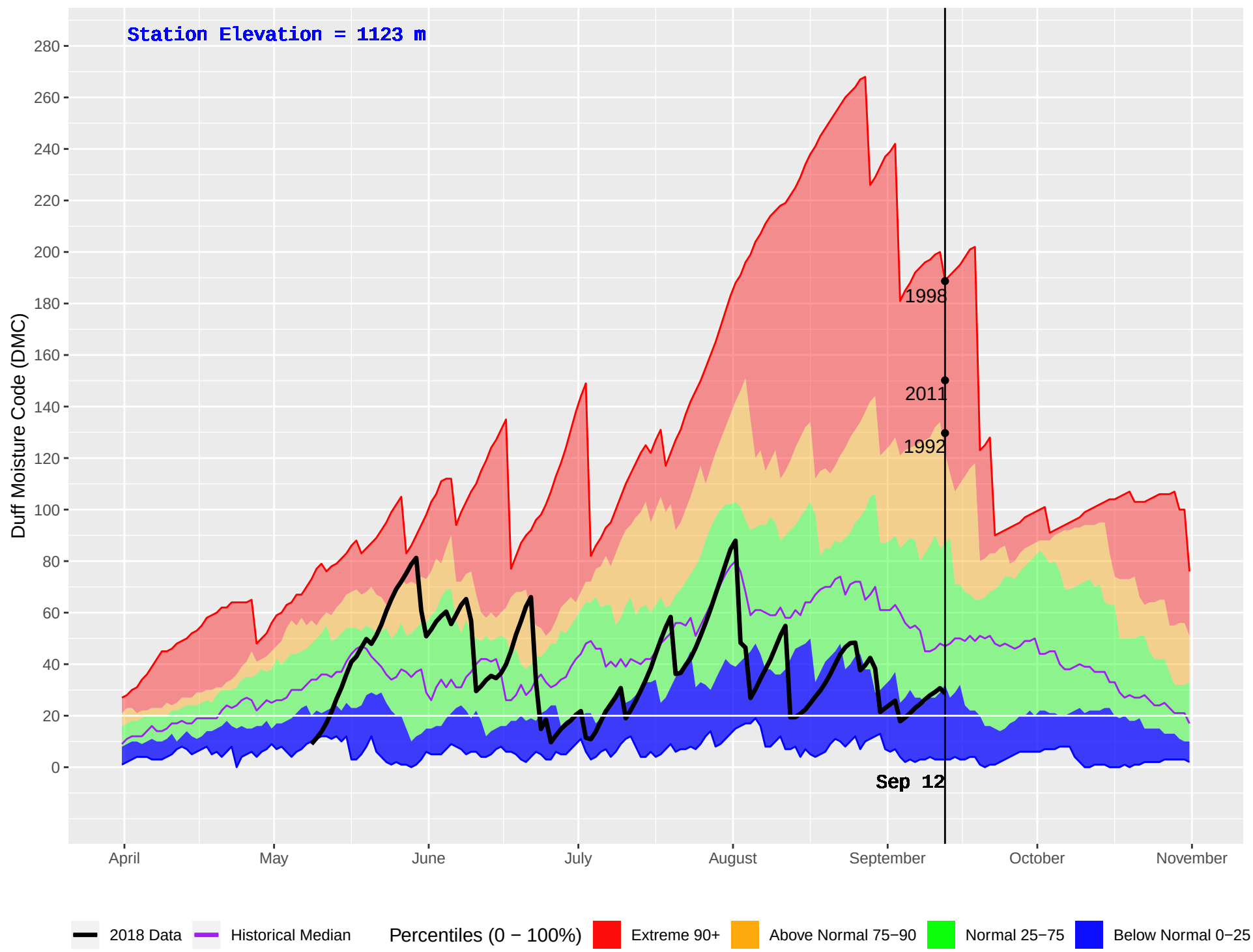
MCLEAN LAKE (311) : Historical (1987–2016) and Current (2018) Daily Duff Moisture Code (DMC)
