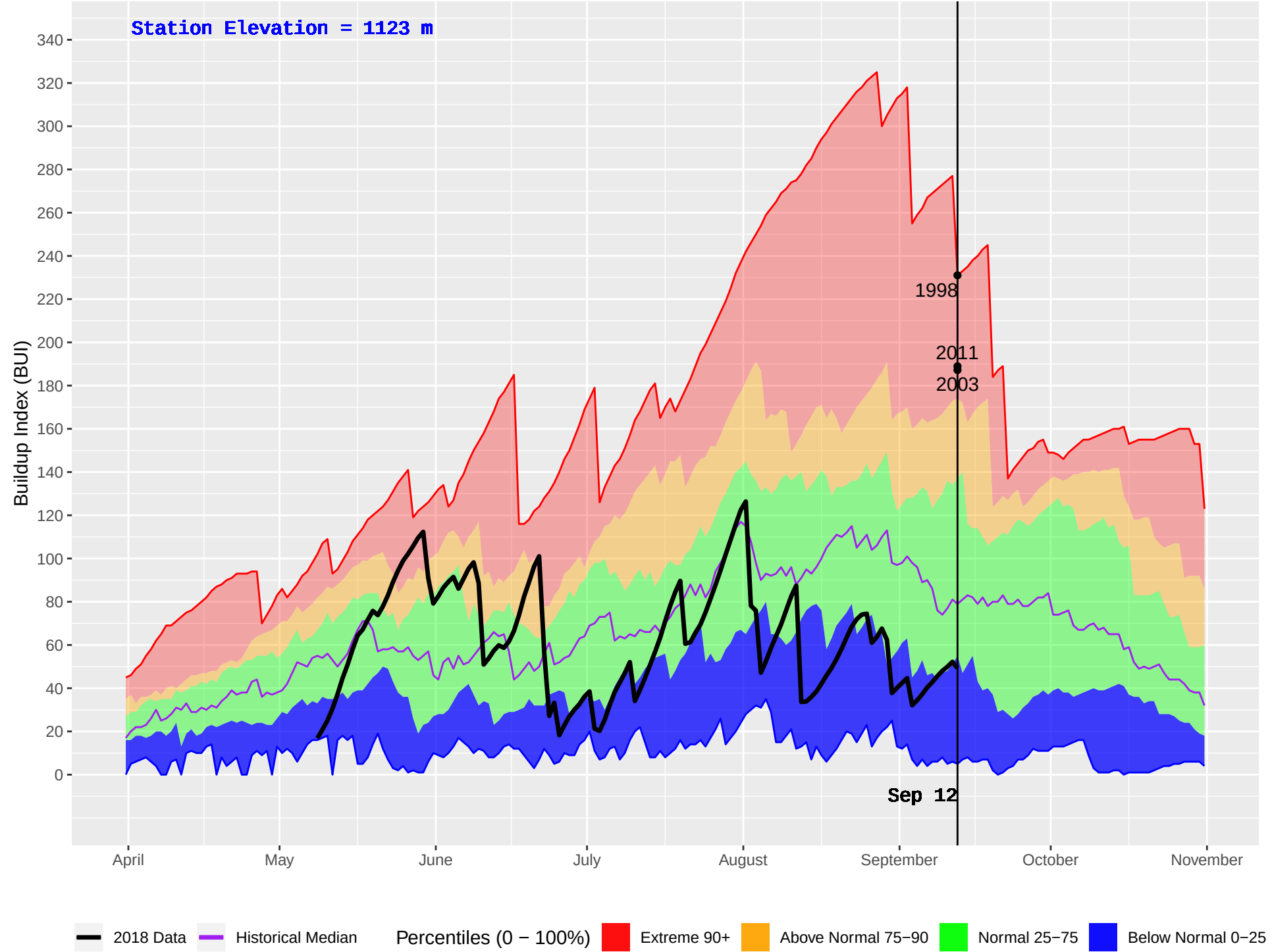
MCLEAN LAKE (311) : Historical (1987–2016) and Current (2018) Daily Buildup Index (BUI)
