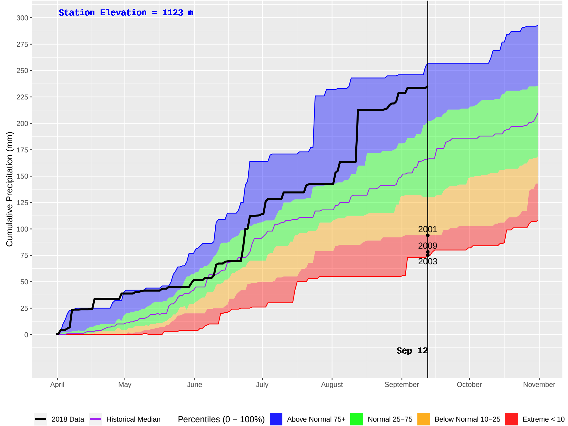
MCLEAN LAKE (311) : Historical (1987–2016) and Current (2018) Daily Cumulative Precipitation
