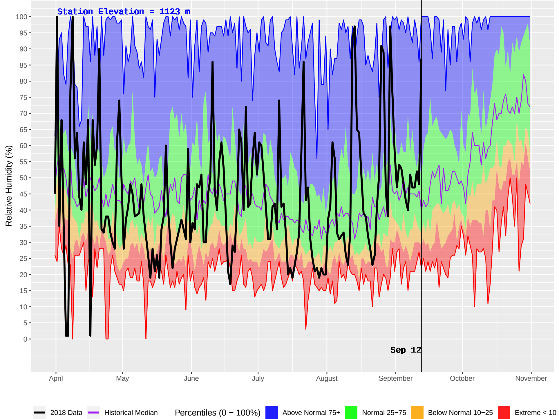
MCLEAN LAKE (311) : Historical (1987–2016) and Current (2018) Daily Relative Humidity
