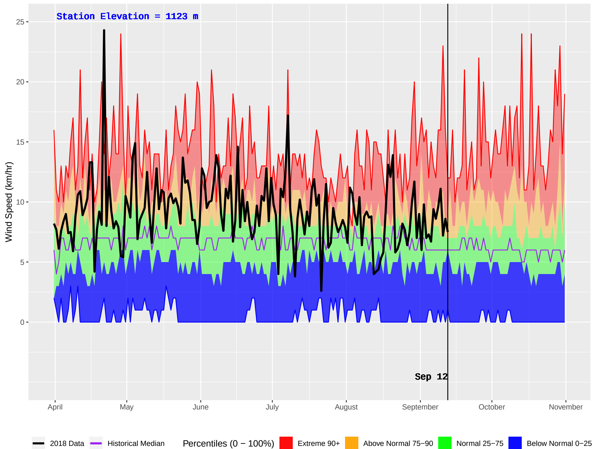
MCLEAN LAKE (311) : Historical (1987–2016) and Current (2018) Daily Wind Speed
