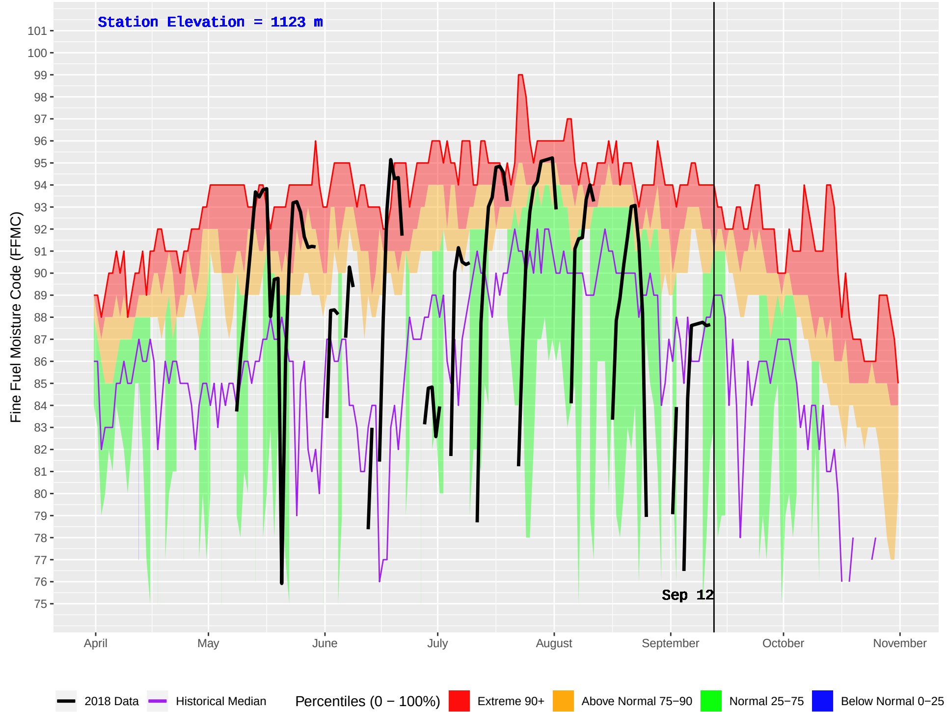
MCLEAN LAKE (311) : Historical (1987–2016) and Current (2018) Daily Fine Fuel Moisture Code (FFMC)
